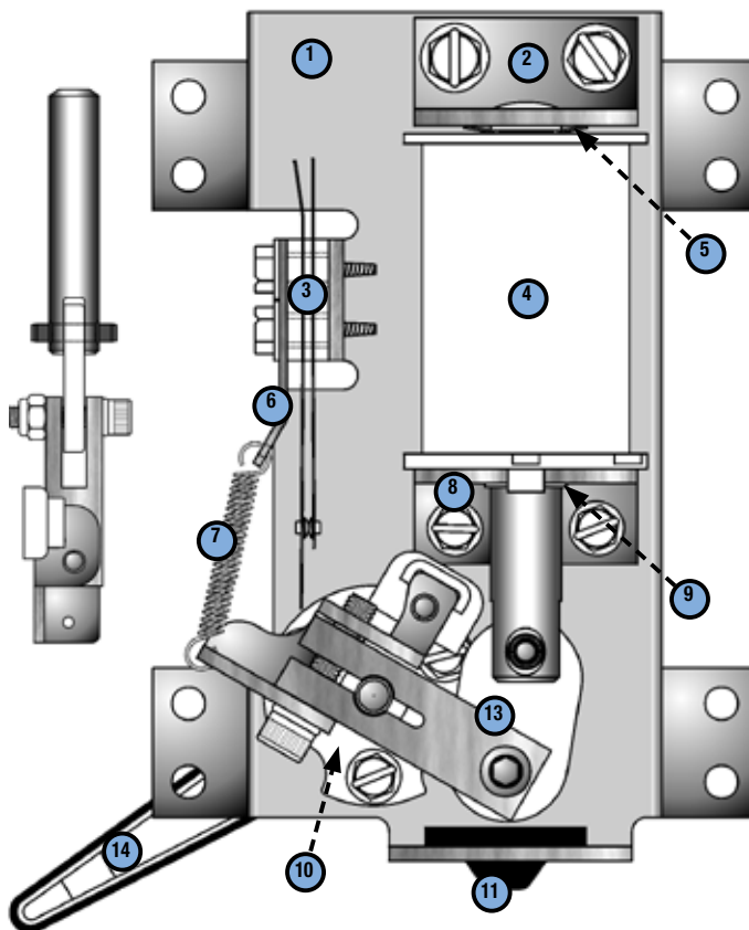
Figure 5.11.1. Right flipper assembly 500-6543-12-ND bottom view.
