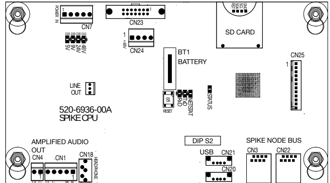
Figure 3.4.1. SPIKE CPU Node connector detail.
