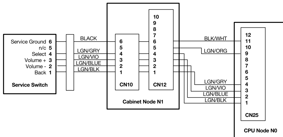
Figure 4.1.1. Service switch wiring. Note that the Cabinet Node must be present and CN10 and CN12 connected for the Coin Door Service Switches to function correctly.
