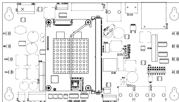
Figure 4.1.1. SPIKE 2 CPU Node connector detail.
