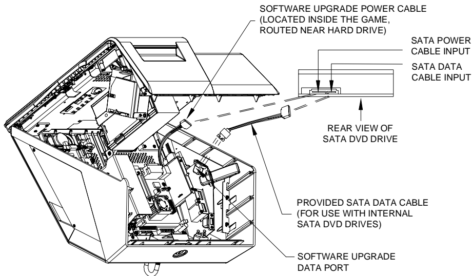
FIGURE B - INTERNAL VIEW OF MEGATOUGH RX
