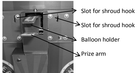
Prize arm and balloon holder mechanism with shroud removed.
