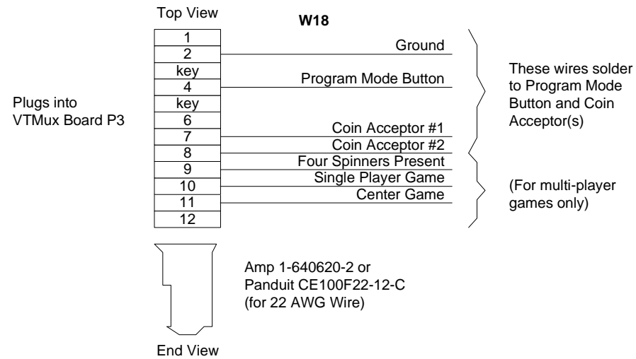
FIGURE 20 VTMUX BOARD P3 TO PROGRAM MODE BUTTON, SINGLE PLAYER, AND COIN ACCEPTOR
