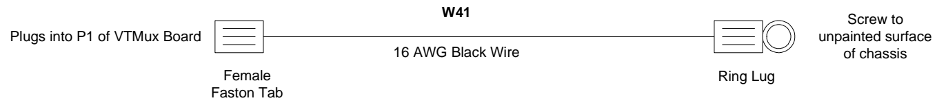
FIGURE 27 - AUDIO GROUND
