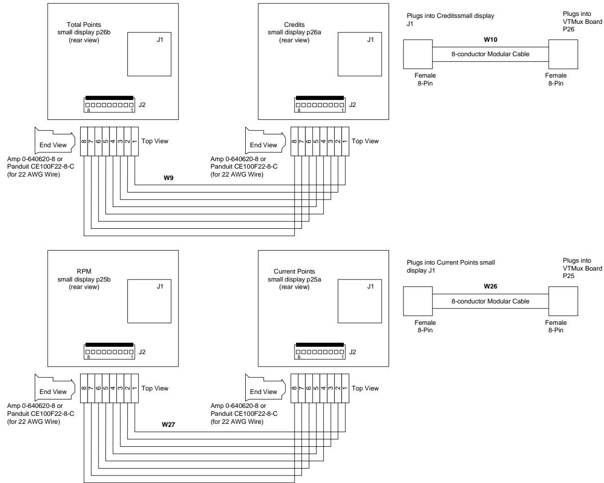
FIGURE 28A VTMUX BOARD P26 TO CREDITS SMALL DISPLAY J1 FIGURE 28B VTMUX BOARD P25 TO CURRENT POINTS SMALL DISPLAY J1
