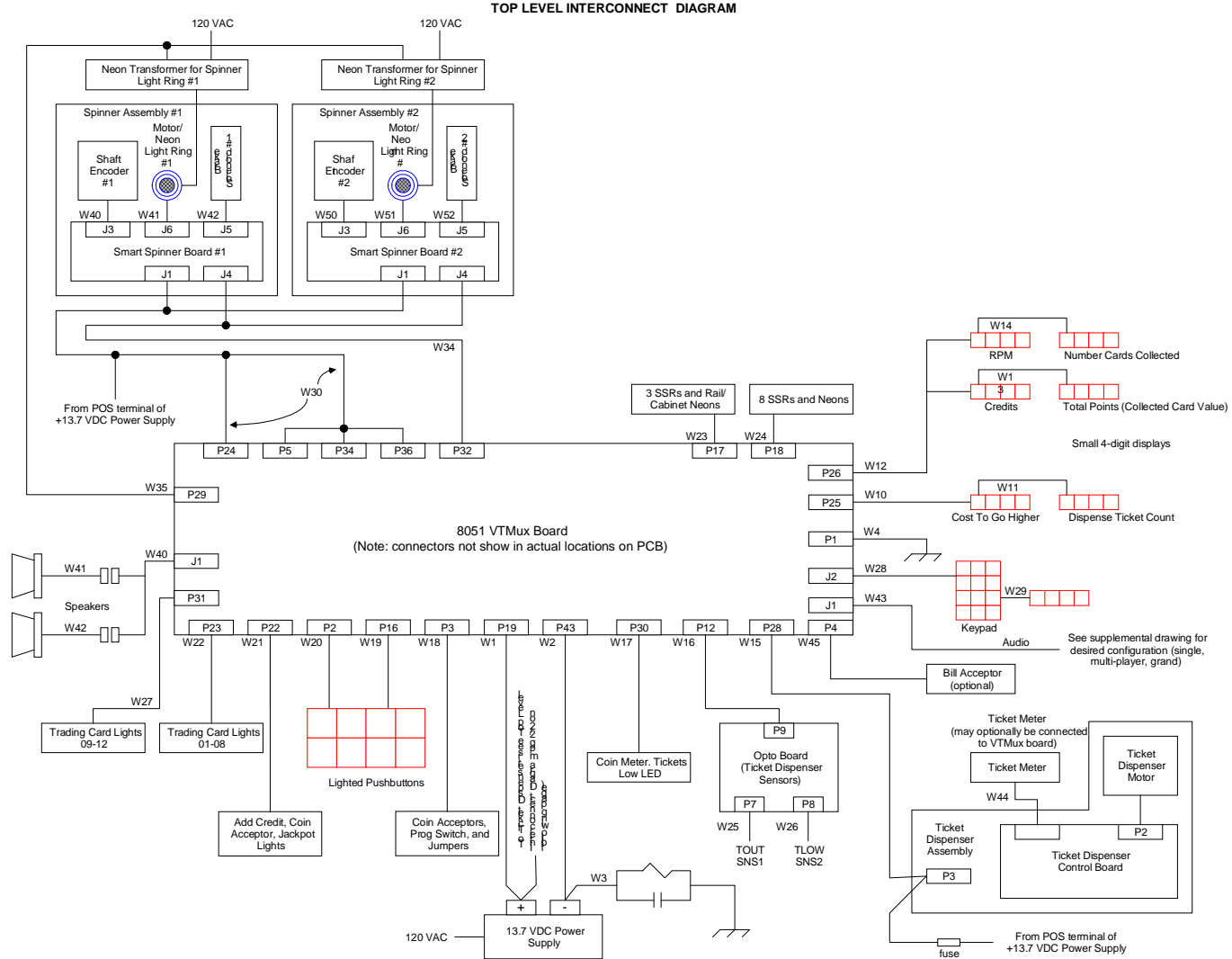
FIGURE 1 – TOP LEVEL INTERCONNECT DIAGRAM
