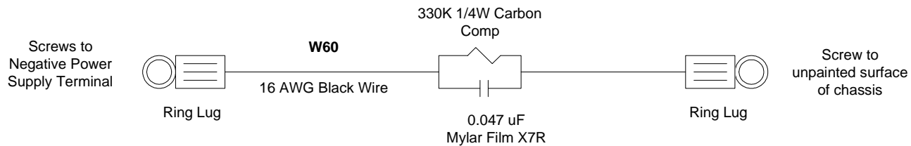
FIGURE 26 CHASSIS GROUND
