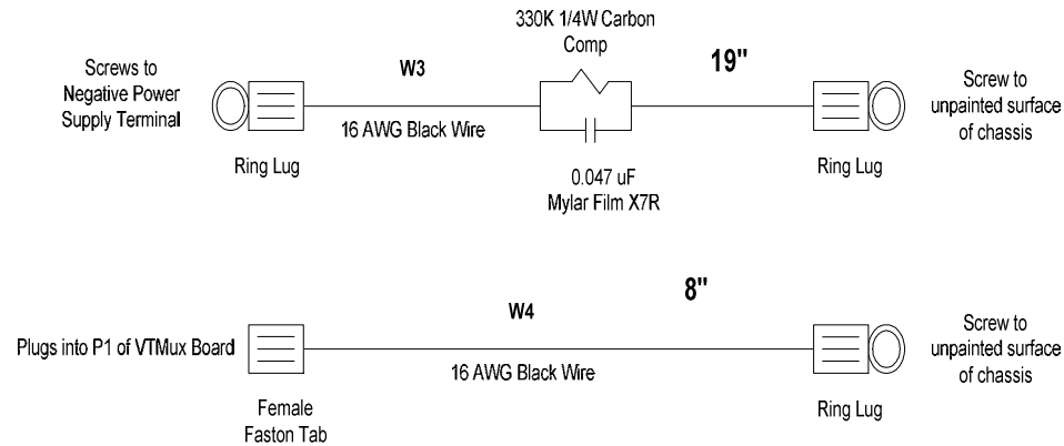
Figure 19 Topper Lights Wiring
