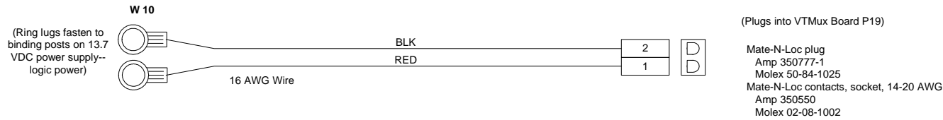
FIGURE 24 13.7 VDC POWER SUPPLY TO 8051 VTMUX BOARD P19
