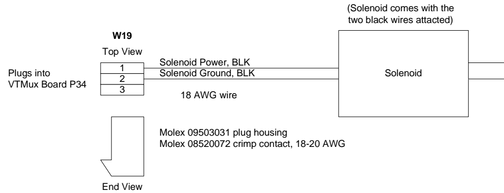
FIGURE 16 VTMUX BOARD P34 TO BRAKE SOLENOID
