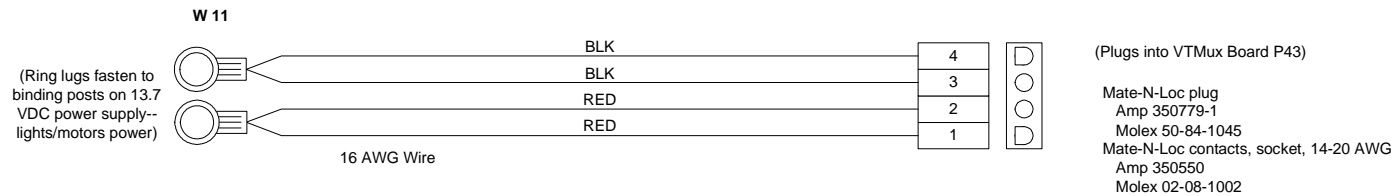
FIGURE 25 -13.7 VDC POWER SUPPLY TO 8051 VTMUX BOARD P43
