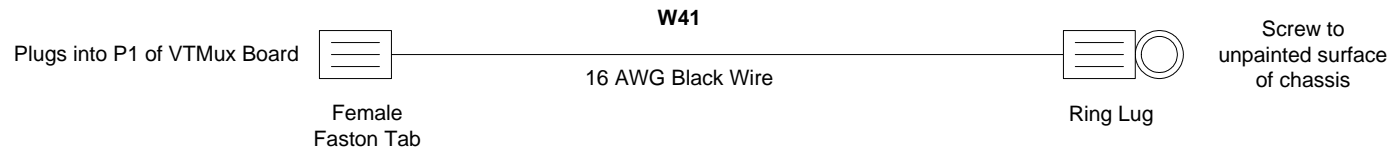
FIGURE 21 - AUDIO GROUND
