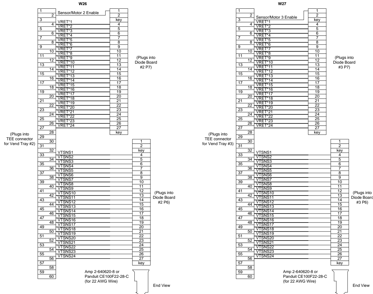
FIGURE 21A 60-PIN RIBBON CABLE TEE TO DIODE BOARD #2 P7
