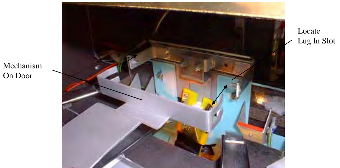
Moving Coin Entry Mechanism
