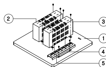
8-6. POWER PANEL ASS'Y
