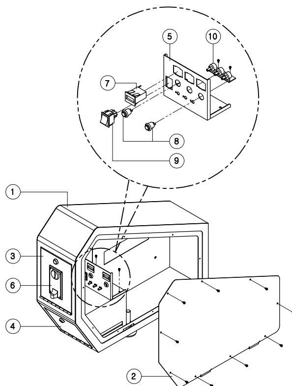
8-4. COIN BOX ASS'Y
