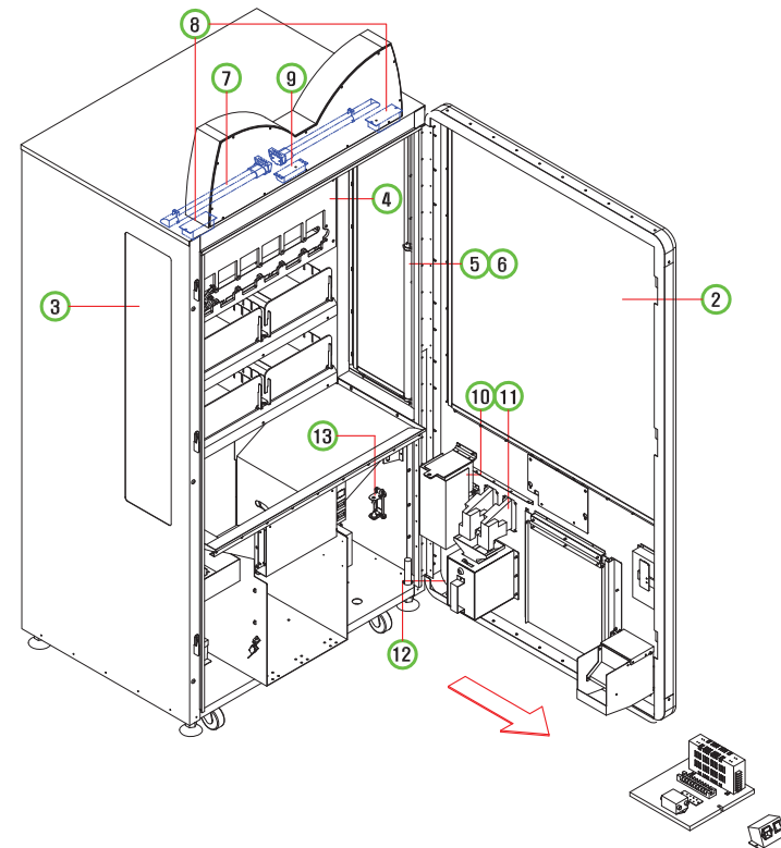
1 MAIN CABINET PART
