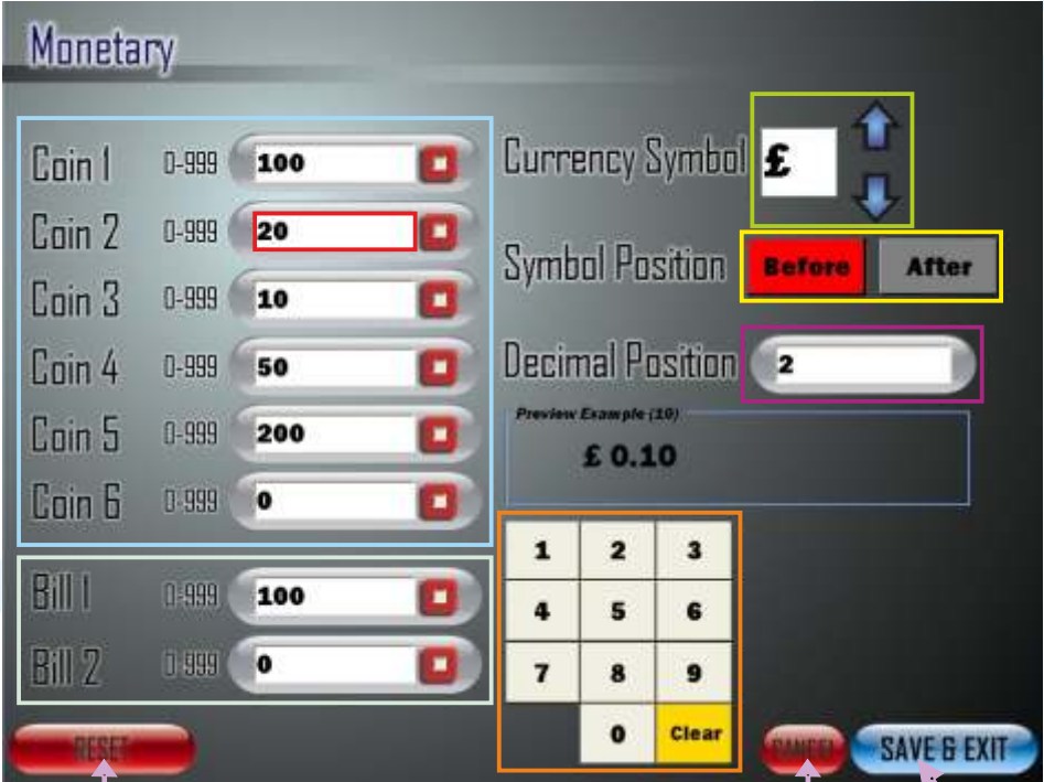
fig. 2.1 - Monetary screen
