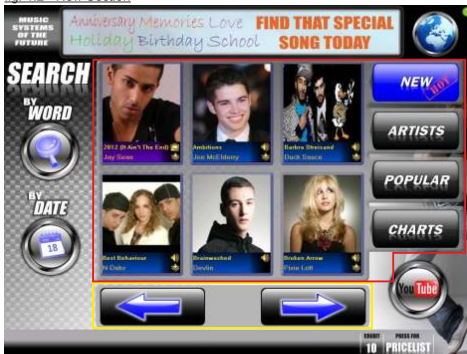
fig. 1.2 - New Section
