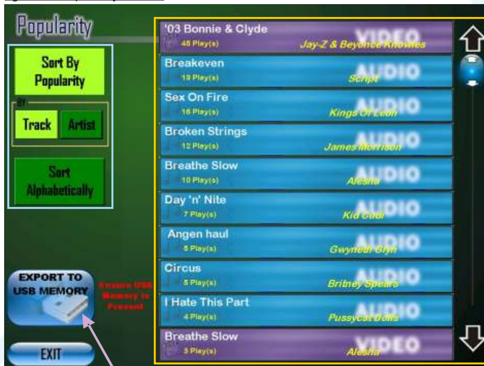
fig. 2.4 - Popularity screen
